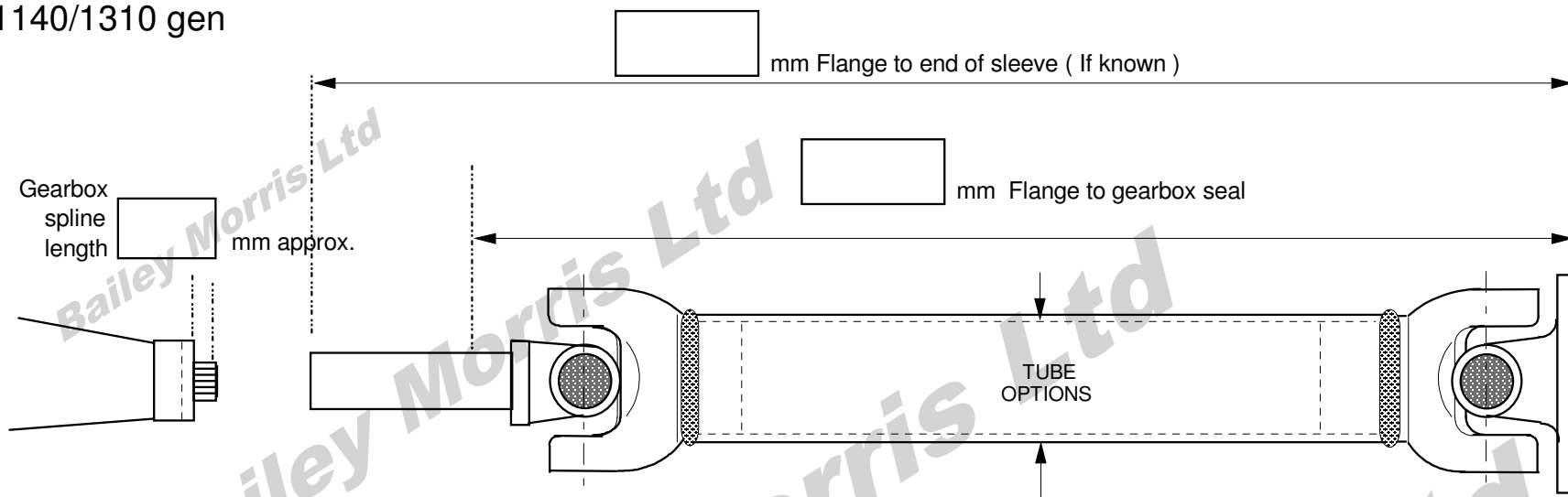
Gearbox Sleeve
